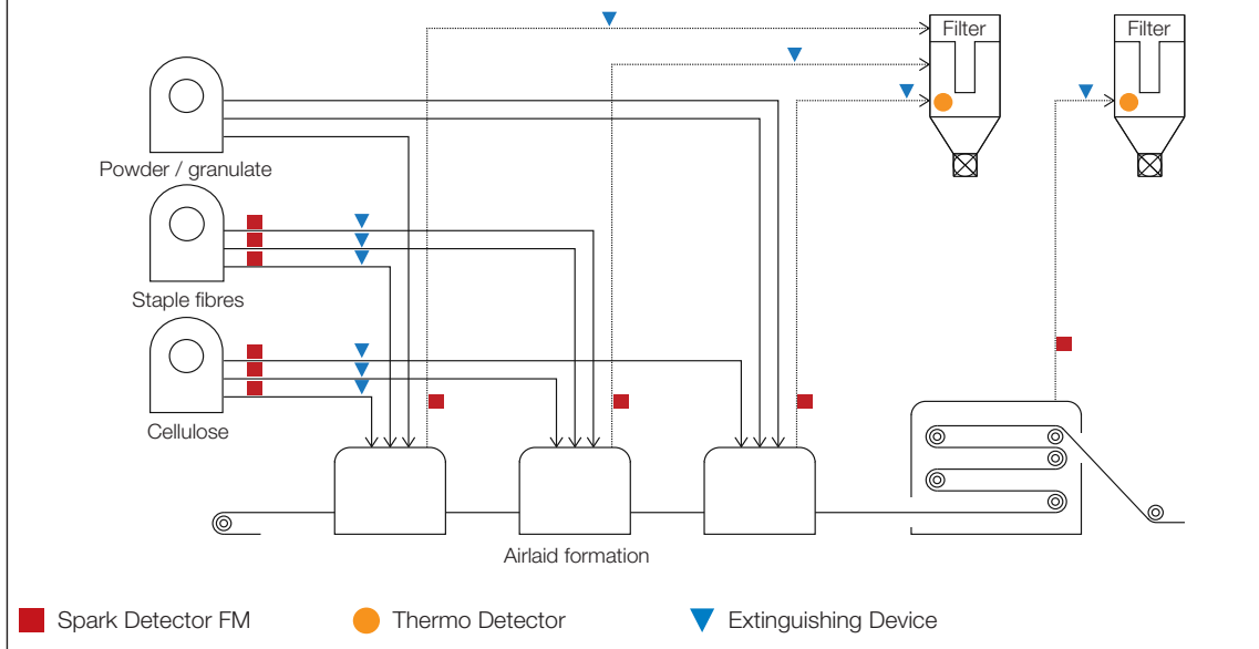
Diagram of protection concept for the hygiene industry
